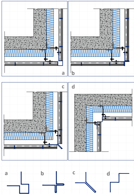
CORNER FLASHINGS
