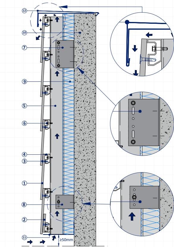
VENTILATED PROFILE AND TOP FLASHING
