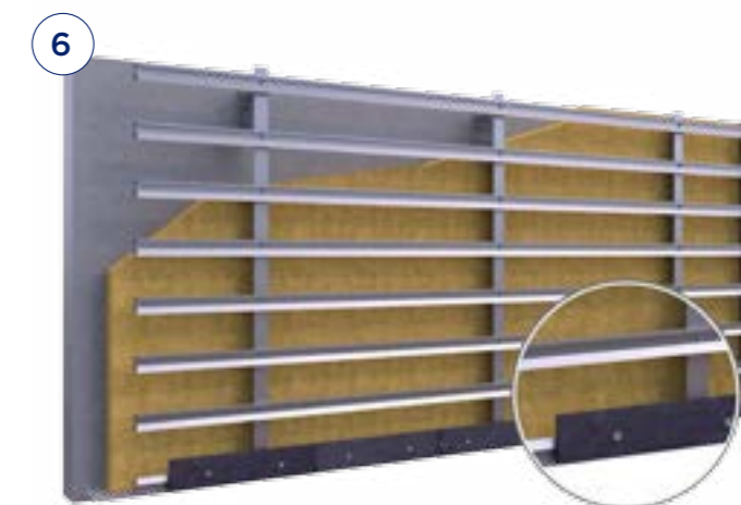
Fixing the first course slate
